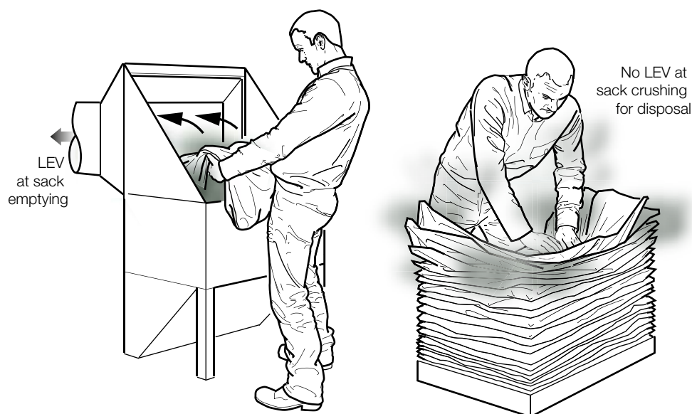
Figure 6 An LEV system to control dust from sack emptying but uncontrolled sack disposal
