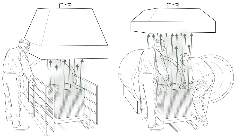
Figure 27 Canopy hoods over a hot process
