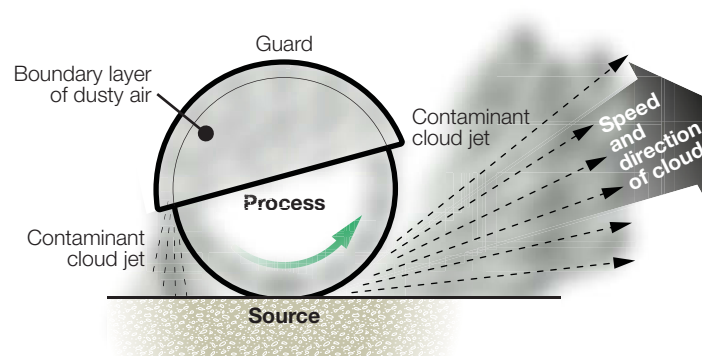
Figure 4 The source and contaminant cloud concepts for an angle grinder
