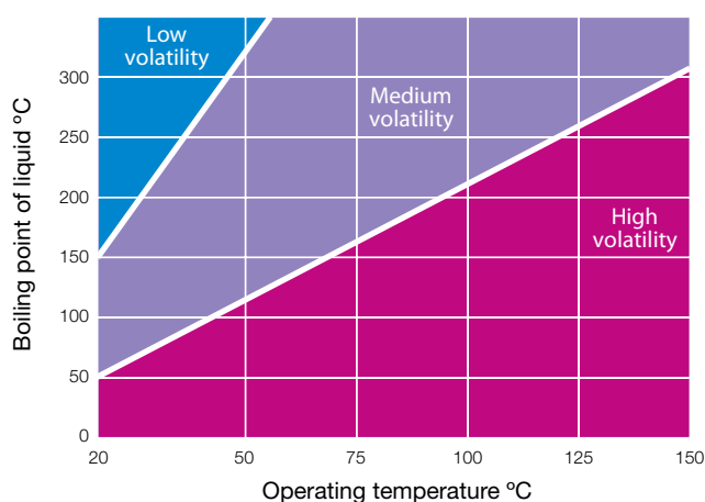
Figure 49 Graph to select volatility of liquid
