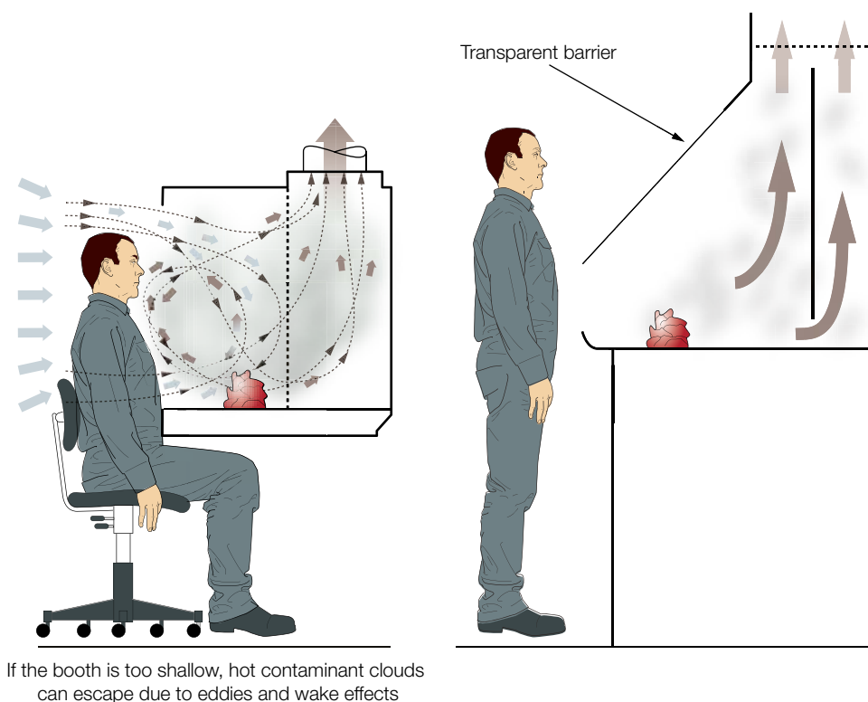
Figure 21 Partial enclosing hood showing wake in front of worker's body
