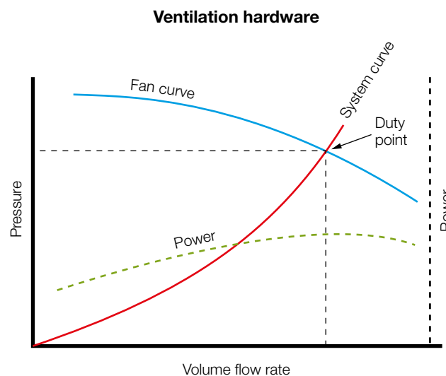
Figure 35 Fan curve showing intersection with system curve
