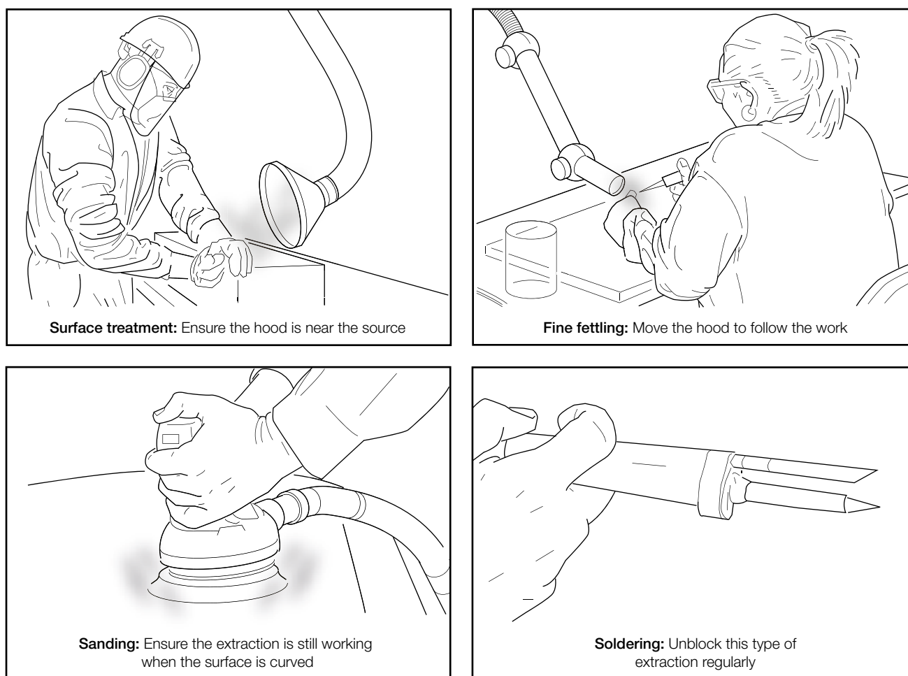
Figure 30 Some capturing hoods
