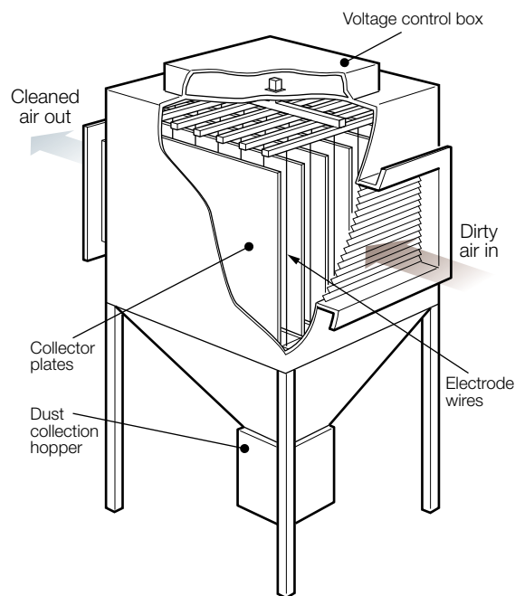
Figure 38 Electrostatic precipitator
